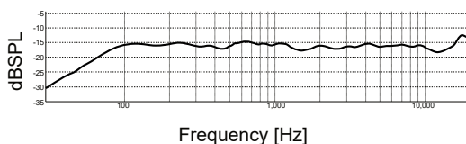
Frequency response
