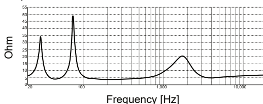
Impedance
