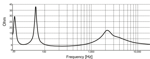
Impedance
